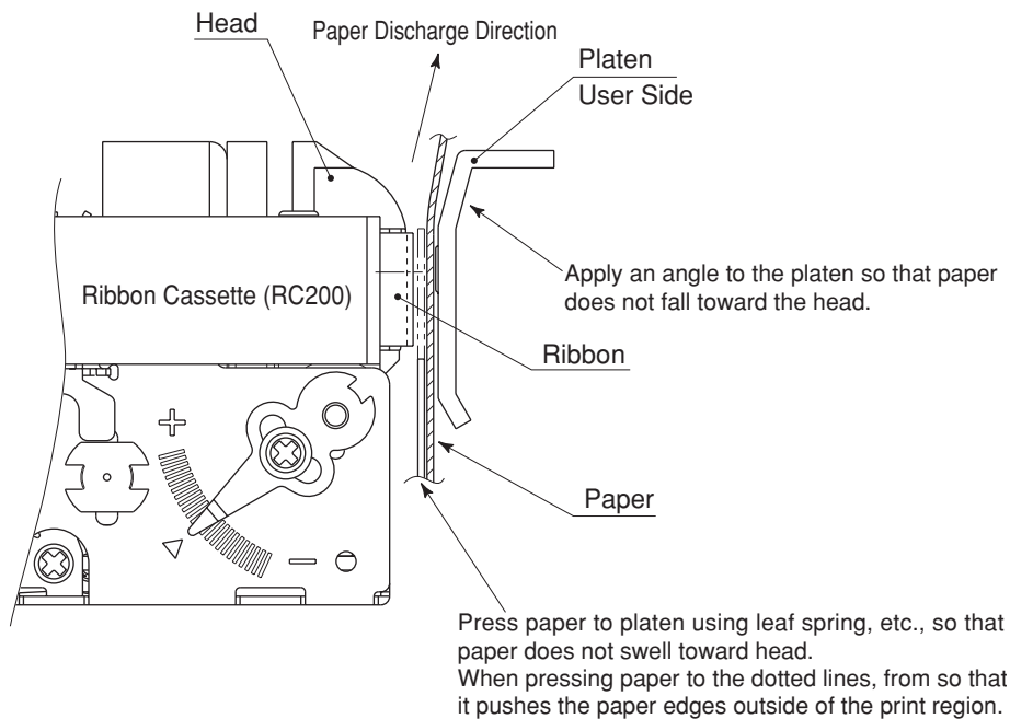
Fig. 5-3 Precautions for Designing the Paper Path
