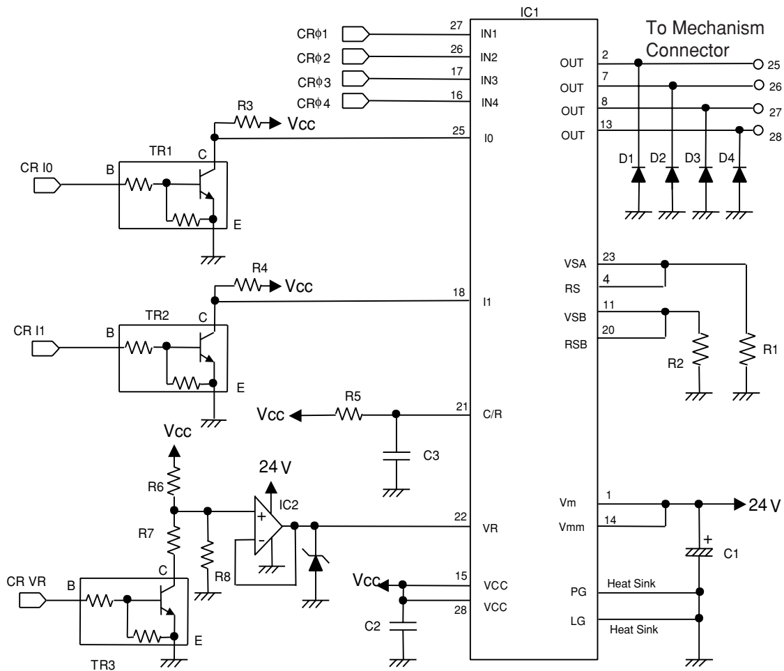
Fig. 4-10 Drive Circuit
